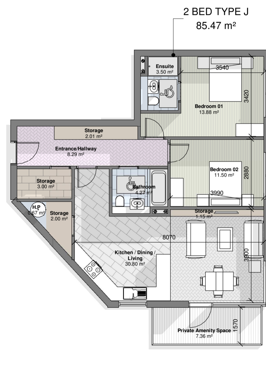
2 BEDROOM APARTMENT TYPE J 1 : 100
