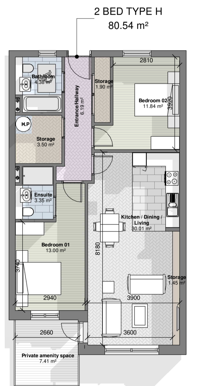
2 BEDROOM APARTMENT TYPE H 1 : 100
